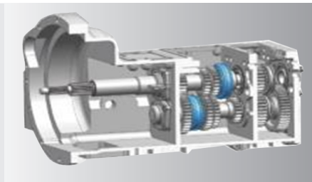
12+12 shuttle gears
