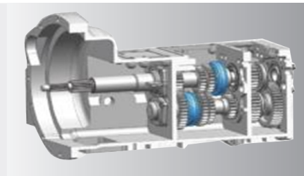
12+12 shuttle gears
