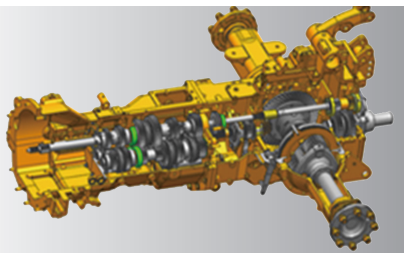
Optional Power shuttle transmission
